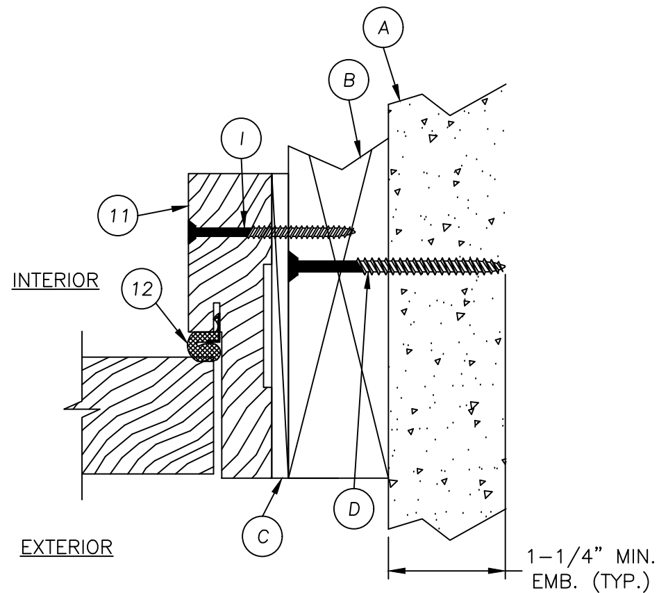
2 HORIZONTAL CROSS SECTION 3
